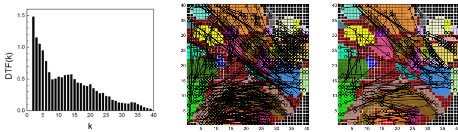
Fig. 2: 40×40 SOM of the LCVF data. Left: The DTF. Middle: Visualized in the cluster map are all 521 violating connections with strengths above 15. Right: Visualized are the 165 inter-cluster violating connections with strengths above 15.
