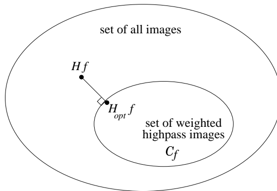
Figure 2: The projection of the highpass filtered image Hf onto the set of all weighted highpass filtered images C_f defined in (6) yields the optimal weighted highpass filtered image H_{opt}f .
