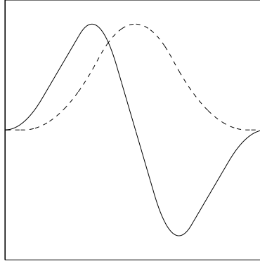
Figure 1: Smoothing function \phi (dashed) and wavelet \psi (solid) employed in the multiscale decomposition.
