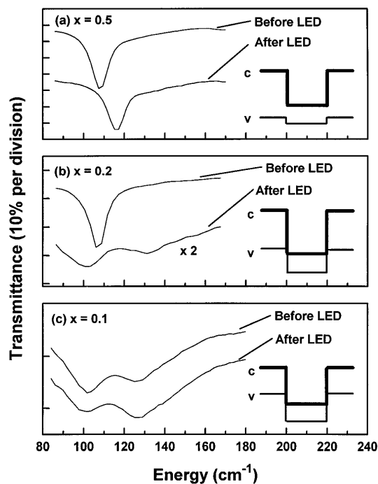
FIG. 1. Transmission spectra at 4 T before and after exposure to an in situ red LED: (a) x = 0.5 , (b) x = 0.2 , and (c) x = 0.1 . Insets show schematically the ideal (charge transfer or band bending not included) conduction (thick lines) and valence (thin lines) band lineups for the three samples.
