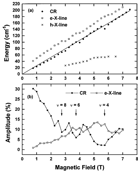
FIG. 2. Results for a sample with x = 0.1 after exposure to a red LED. (a) Energy vs magnetic field for the three lines at 4.2 K. The straight line has a slope corresponding to m^* = 0.0352m_0 . (b) Plot of percent change in transmittance at peak of the two lines vs magnetic field.
