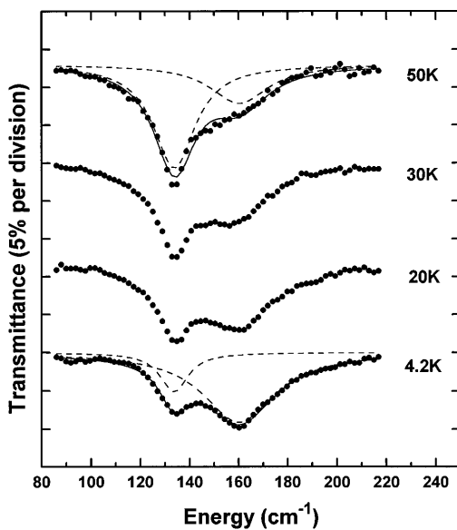
FIG. 3. Temperature dependence of the two lines for a sample with x = 0.1 after exposure to the LED. Ratios of transmitted intensity at the indicated temperature and B = 5 T to a background spectrum (at the same temperature and B = 0 ) are shown by the dotted curves. Individual Lorentzian lines fitted to the data (dashed lines); overall fit (solid lines).
