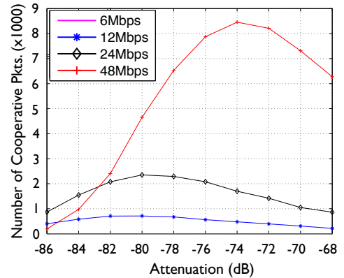
Fig. 4. Number of cooperative NvMISO packet transmissions for different rates.
