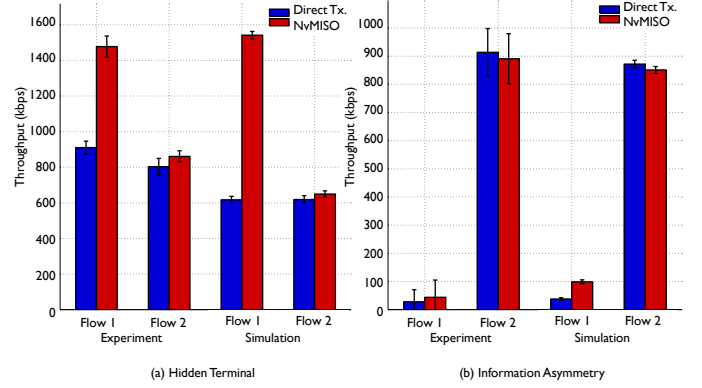
Fig. 10. Cooperation in Hidden Terminal (a), and Information Asymmetry (b) Topologies
