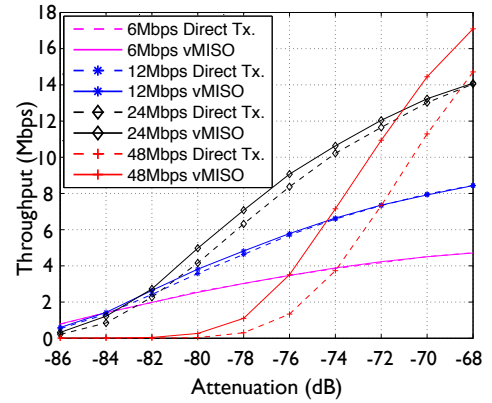
Fig. 3. Throughput of NvMISO for different transmission rates.
