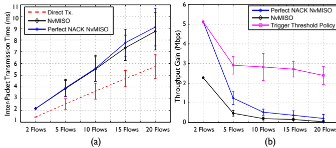
Fig. 13. (a) Mean packet inter-transmission time for different network sizes. (b) Per-flow throughput gains/losses for different network sizes
