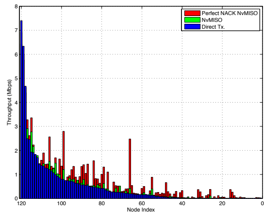
Fig. 14. Network consisting of 120 flows.
