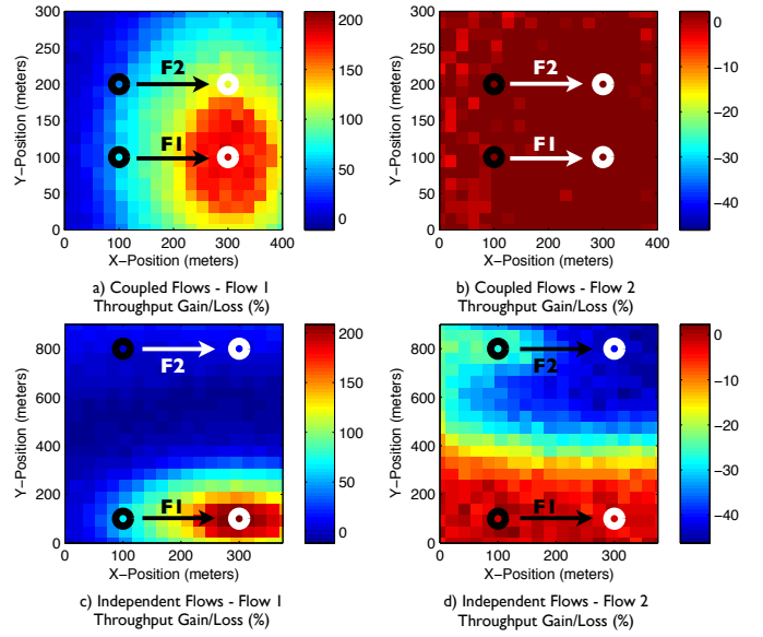
Fig. 12. Influence of helper's transmission footprint in coupled and uncoupled flows as a function of its position.
