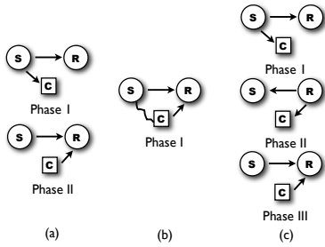
Fig. 1. Operation of vMISO protocols. Sender transmits to a receiver with the help of a vMISO cooperator node.
