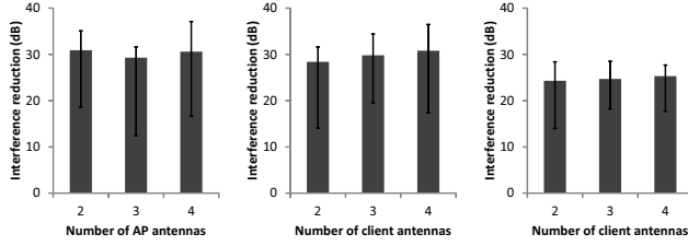
Figure 6: Interference reduction from interference cancellation by the AP (Left), interference cancellation by the client (Middle), and interference alignment by the client (Right). On average interference cancellation and interference alignment achieve 30 dB and 25 dB interference reduction, respectively. The number of AP or client antennas does not have an obvious impact on the cancellation or alignment accuracy.
