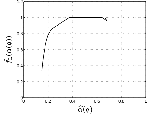
Figure 4. Wavelet-based Legendre spectrum estimator (13) averaged over 100 independent realizations of a generalized Weierstrass process [8] W(t) := \sum_k \lambda^{-kH_t} \sin(\lambda^k t + \phi_k) with \phi_k uniform random variables on [0, \pi] . The Hölder function H_t grows linearly from H_0 = 0.2 to H_1 = 0.8 .
