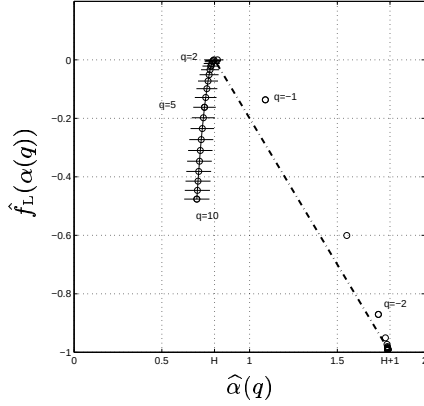
Figure 3. Empirical statistics on \widehat{f}_L(\alpha(q)) plotted versus \widehat{\alpha}(q) for fBm. The dashed dot line corresponds to the theoretical Legendre spectrum. The error bars denote the standard deviation on the estimates \widehat{\alpha}(q) . Experimental conditions are identical to those of Figure 1.
