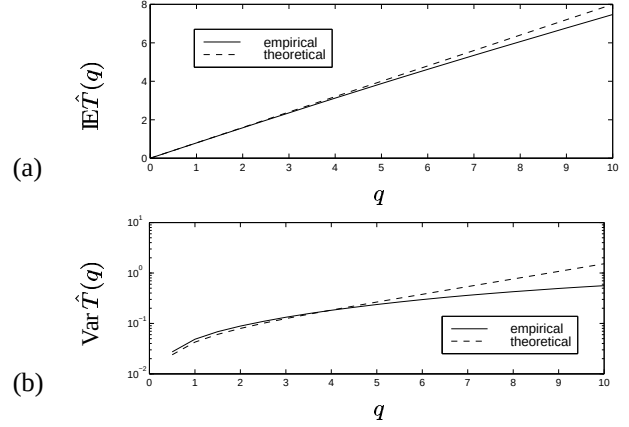
Figure 1. Statistics of the estimator \hat{T}(q) versus q . (a) \mathbb{E} \hat{T}(q) ; (b) \log \text{Var} \hat{T}(q) . Numerical results based on 1000 realizations of an fBm (exact Cholesky synthesis algorithm) with H = 0.8 and N = 1024 and a Daubechies wavelet with three vanishing moments.
