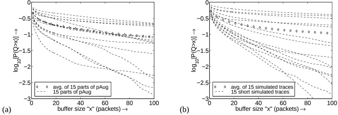
Figure 5: Here we partition the pAug trace into 15 sub-traces of equal number of packets and compare their queueing behavior with that of 15 synthesized traces of the same length. In (a), observe that the sub-traces have a wide variation in tail queue behavior. In (b), observe that the synthesized traces display a similar variation in tail queue behavior as the sub-traces.
