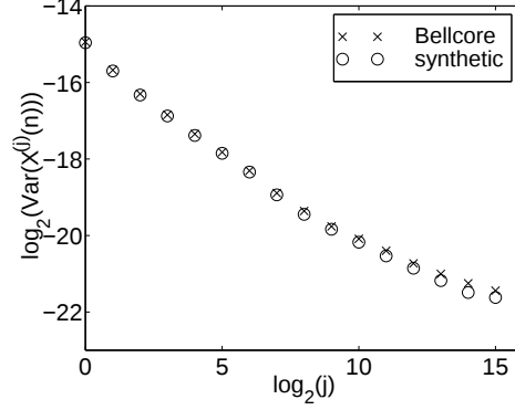
Figure 4: Variance-time plot of the Bellcore data “x” and one realization of the \beta MWM synthesis “o”.
