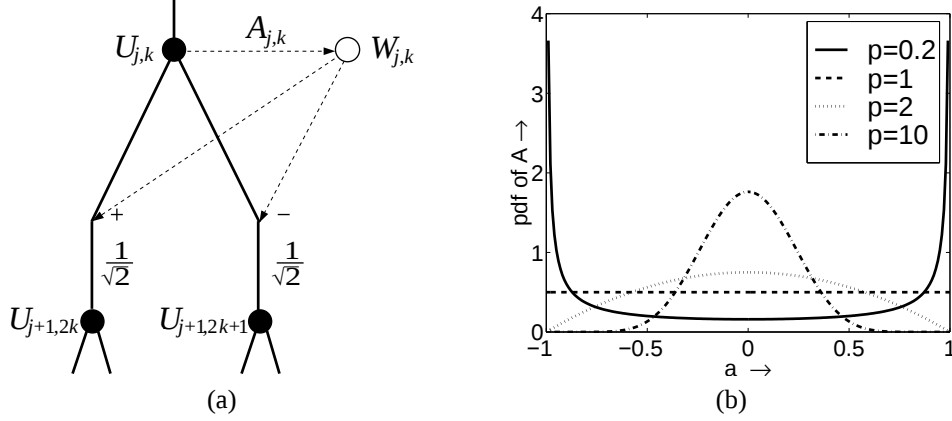
Figure 2: (a) MWM construction: At scale j , we form the wavelet coefficient as the product W_{j,k} = A_{j,k}U_{j,k} . Then, at scale j+1 , we form the scaling coefficients U_{j+1,2k} and U_{j+1,2k+1} as sums and differences of U_{j,k} and W_{j,k} (normalized by 1/\sqrt{2} ). (b) Probability density function of a \beta(p, p) random variable A . For p = 0.2 , A resembles a binomial random variable, and for p = 1 it has a uniform density. For p > 1 the density appears like a truncated Gaussian density, and as p increases, the density resembles a Gaussian density more and more closely.
