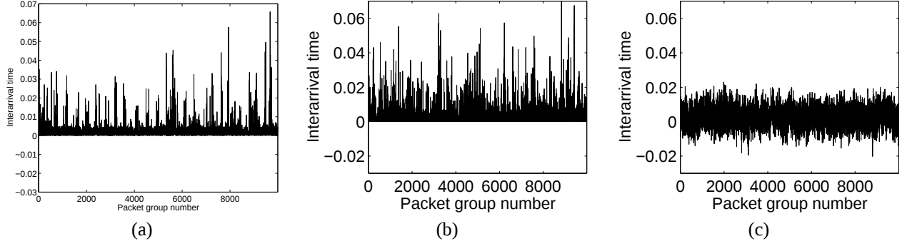
Figure 3: Interarrival times of packets of (a) Bellcore August 1989 [2], (b) one realization of the beta multifractal wavelet model ( \beta MWM) synthesis and (c) one realization of an fGn model. The \beta MWM trace resembles the Bellcore data closely, while the fGn data does not.
