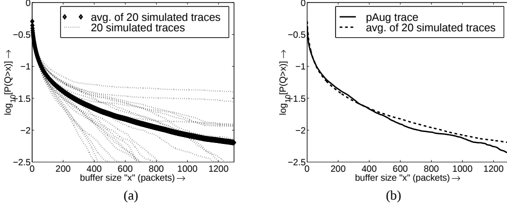
Figure 6: Comparison of the queuing behavior of the Bellcore pAug with that of 20 synthesized \beta MWM traces. Displayed are the tail probabilities of buffer occupancy against buffer size. In (a), observe the variability of the queue performance of the synthesized traces. In (b), observe that the average queue performance of simulated traces and that of the real trace match closely.
