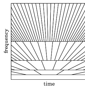
Fig. 3: Warped WT basis tiling.
