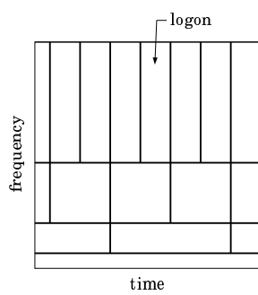
Fig. 2: WT basis tiling.
