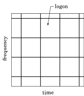
Fig. 1: STFT basis tiling.
