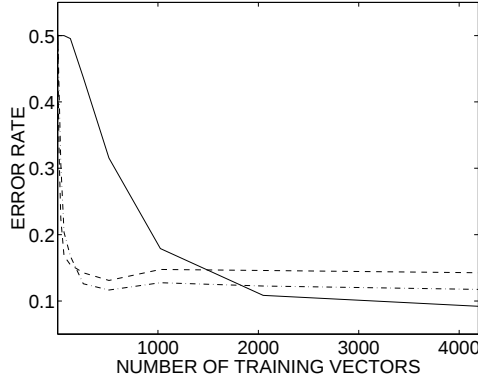
Figure 10: Minimum probability of error rates for quadratic classifier (solid), wavelet-domain IM model classifier (dash), and wavelet-domain HMT model classifier (dash-dot).
