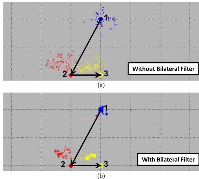
Fig. 17. Continuous gaze tracking demonstration. Each image shows a part of the tablet screen, and the cross-stiches of the grid lines represent the 35 potential ground truth gaze locations. In (a), 3 ground truth gaze locations and the color-coded predicted locations are shown for a single subject from our dataset. Each location is showed in the sequence indicated by the arrows. The distance between the predicted gaze locations and the true gaze location is within the distance between two cross-stiches (3.4 cm). In (b), the predicted locations are passed through a bilateral filter; the fluctuations of the predictions are reduced by the filter.
