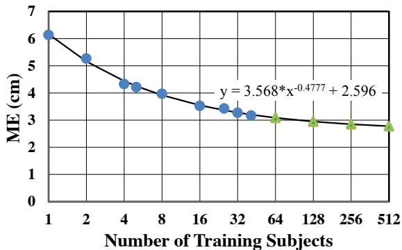
Fig. 14. Effect of training data size on the gaze estimation accuracy of TabletGaze. The round circles are results obtained in the experiment, and a line is fitted to the data points. The triangles are data points derived through extrapolation on the fitted line. We can see that the ME decreases monotonically as the number of training subjects grows larger, indicating that more data could improve the performance further.
