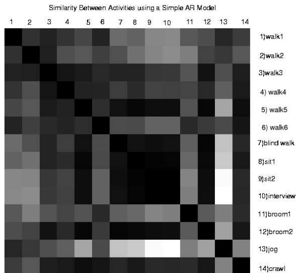
Fig. 10. Similarity matrix for the Mocap data using the AR model
