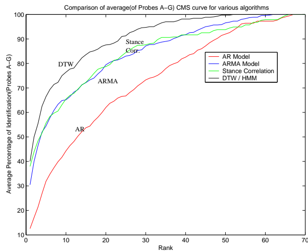
Fig. 4. Average(average of Probes A-G) CMS curves(Percentage of Recognition Vs Rank) using various methods.
