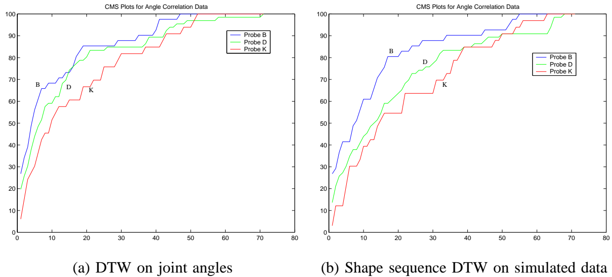
Fig. 6. CMS curve using (a)DTW on joint angles and (b)Shape sequence DTW on simulated data
