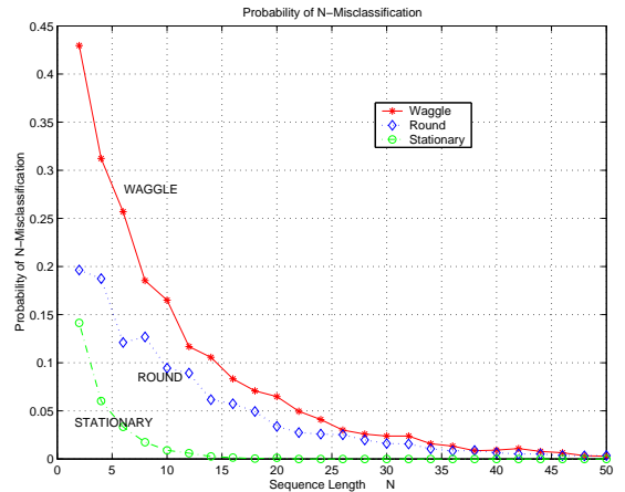
Fig. 4. Probability of N-Misclassification
