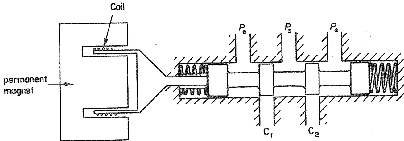
Figure 9.1 Diagrammatic representation of single-stage valve with moving coil armature
