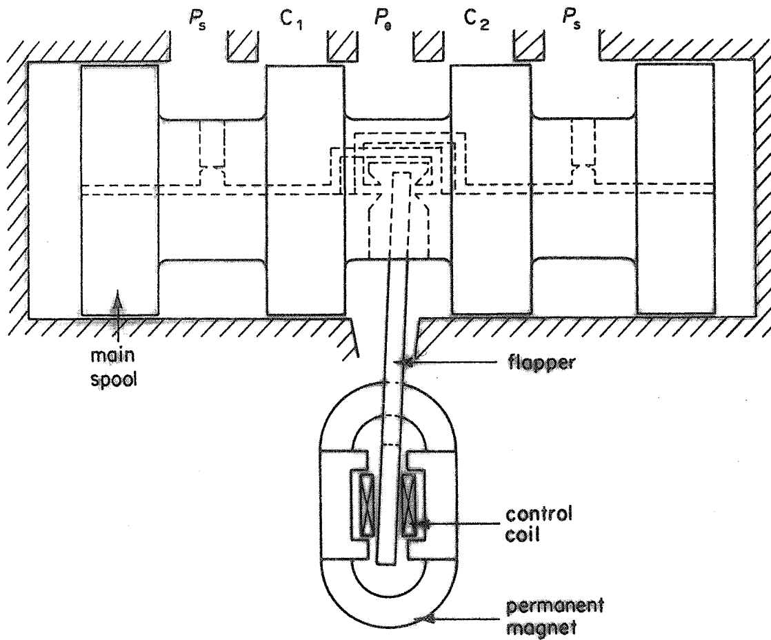
Figure 9.3 Diagrammatic representation of two-stage servo valve with permanent magnet torque motor, flapper-nozzle first stage and position feedback between stages
