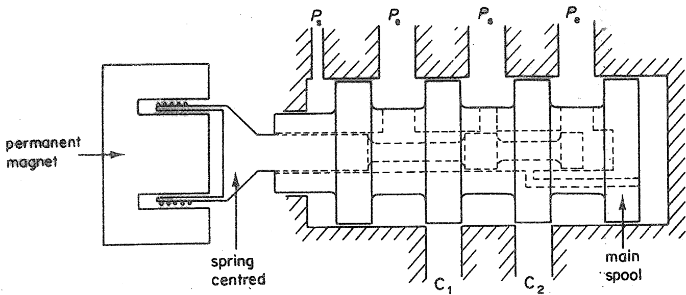
Figure 9.2 Diagrammatic representation of two-stage spool-spool valve
