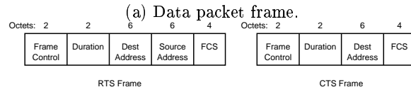
(b) RTS/CTS control packet frames.
